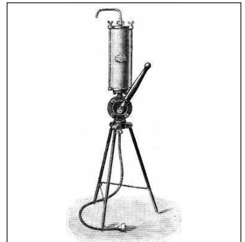
Draagbare Delphin-filter in operationele toestand.
